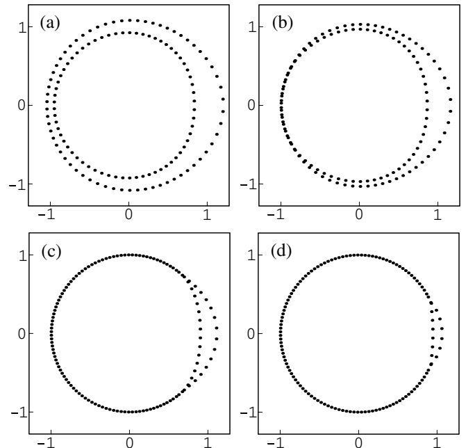
FIG. 1. The 128 zeros of the partition function of the Blume-Capel model in the complex e^h plane, for the 8 \times 8 periodic square grid at e^{-4J} = 1/16 and e^\lambda = (a) 0.9, (b) 0.94, (c) 1, (d) 1.07. The actual zeros lie within a distance of order e^{-10J} + e^{-L/L_0} of those depicted. For \lambda < \lambda_c^- \approx -e^{-4J} , the outer region of the + phase is separated from the inner - phase by an annular region of the 0 phase (a); asymptotically, the zeros lie on the boundaries of these regions. As \lambda increases through \lambda_c^- , the two boundaries coalesce on the left hand side, leading to bifurcation for \lambda > \lambda_c^- . The common boundary grows (c,d) and, eventually, at \lambda = \lambda_c^+ \approx e^{-4J} , the 0 phase disappears and bifurcation terminates. For \lambda > \lambda_c^+ , all zeros lie on the unit circle.
